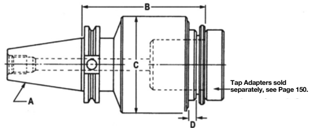
Large Capacity 3/4 thru 2-1/2
