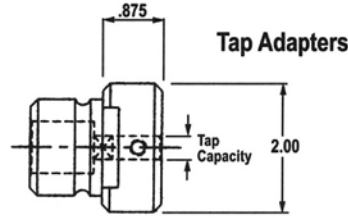
Style #1 Tap Adapters shown on Page 150
